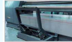
Hydraulically operated side support device
