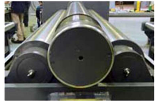
All 4 rolls are manufactured of high quality alloy steel, and hardened to HRC 55 o
