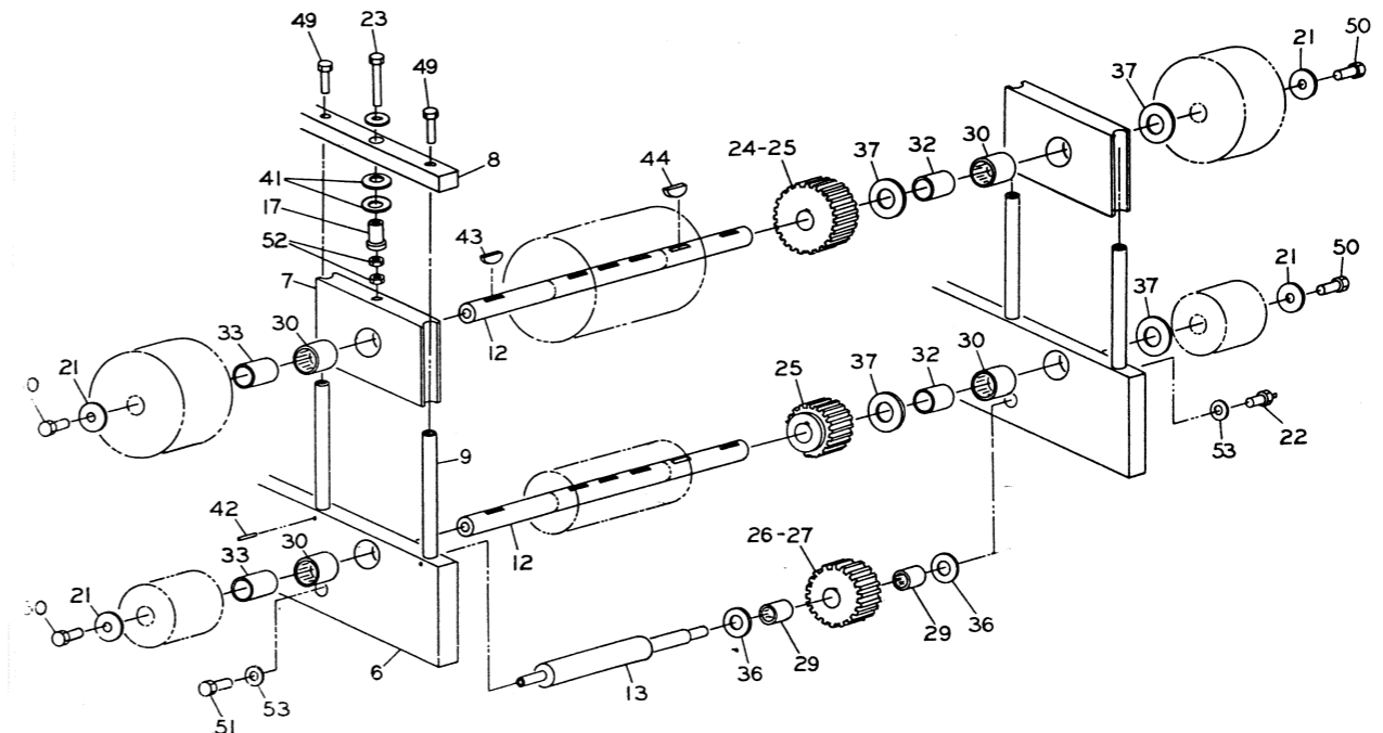
SPINDLE HOUSING ASSEMBLY
