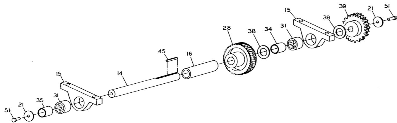
TRANSFER SHAFT ASSEMBLY
